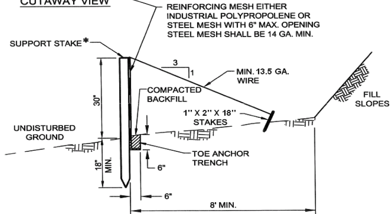
CUTAWAY VIEW
