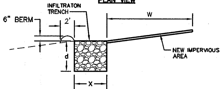
SECTION VIEW
